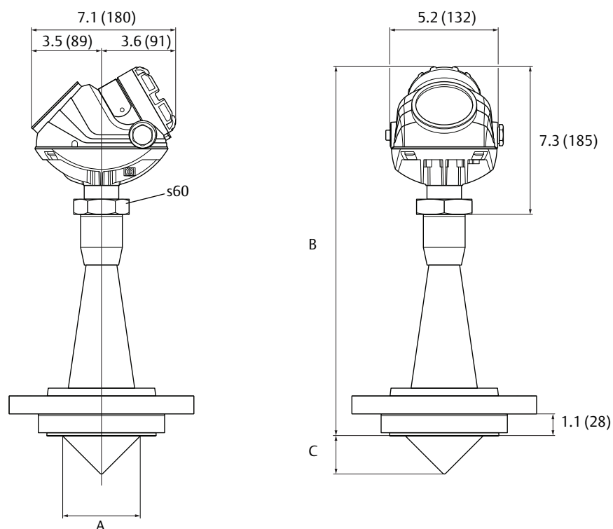
Figure 3. Rosemount 5402 with Process Seal Antenna (Model Codes 2P-4P)
